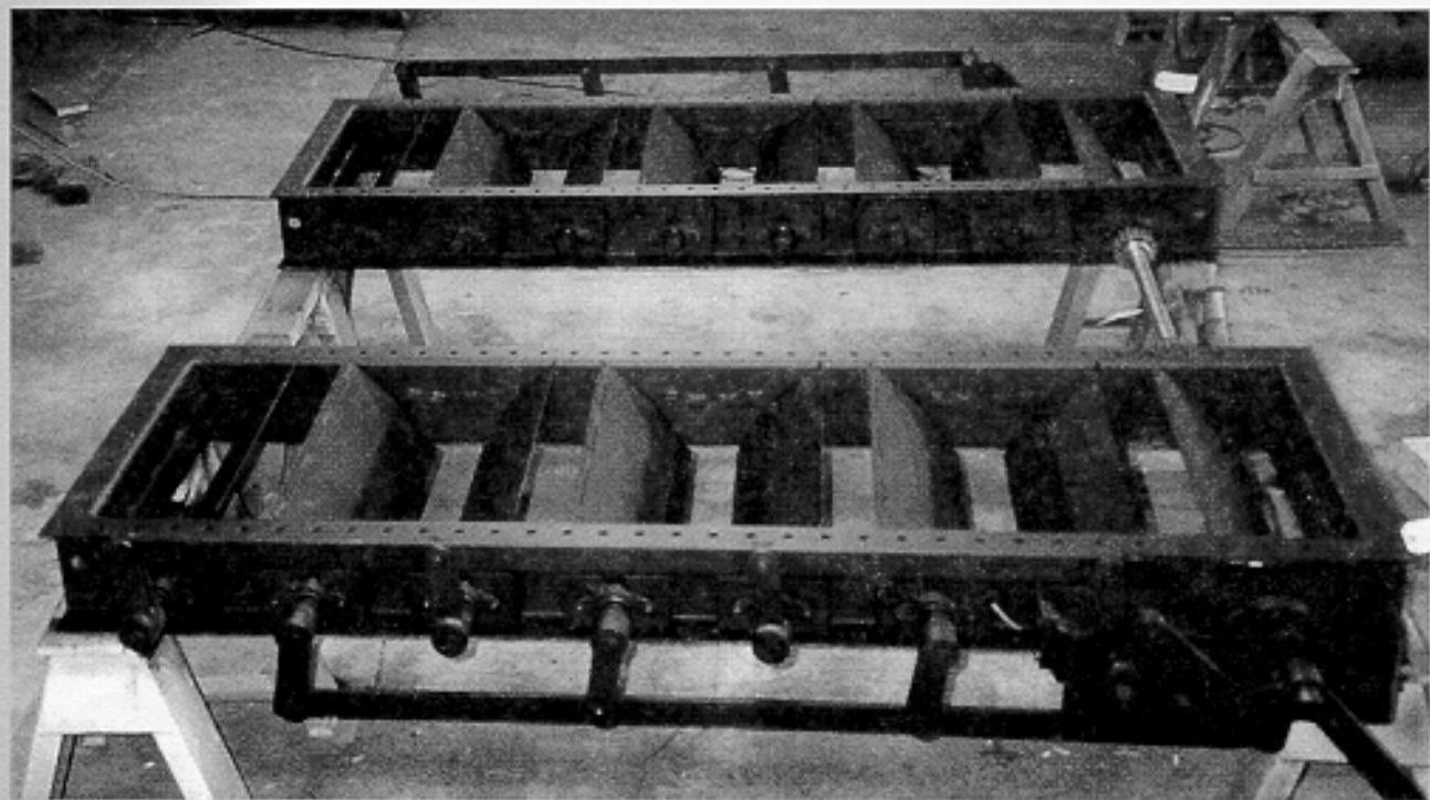
Opposed blade fan outlet louvers in tandem operation.
